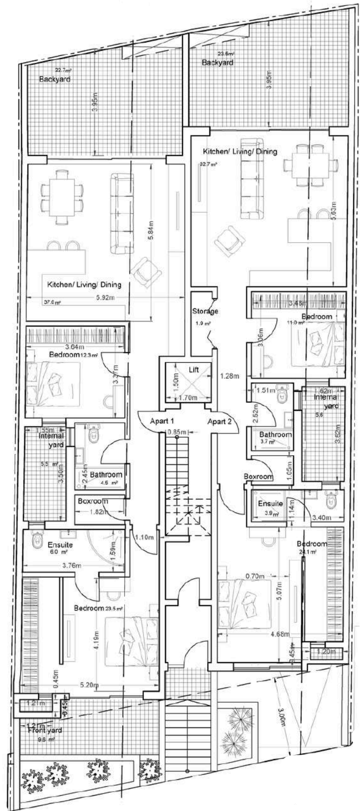
GROUND FLOOR
